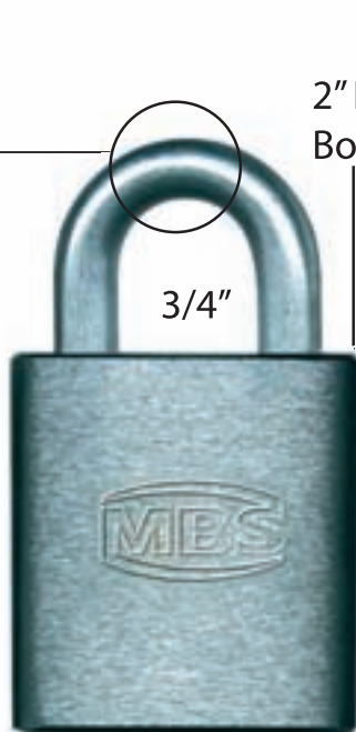
Z6T5 3/4" Shackle
